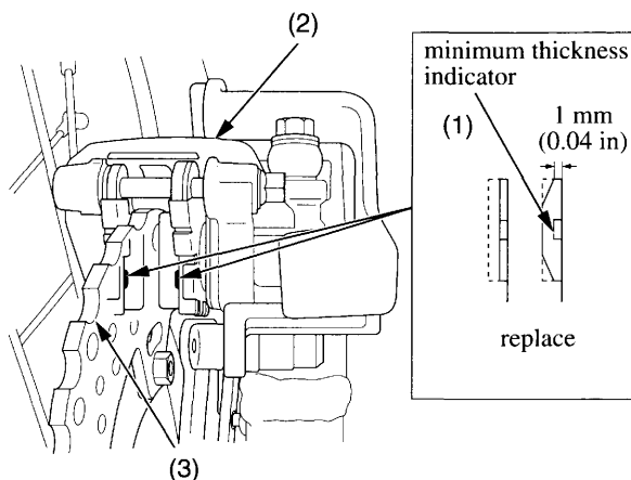
(1) brake pads (2) rear brake caliper
