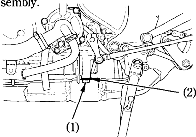
(2) Sealing washer
