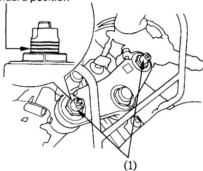
(1) Preload adjuster
