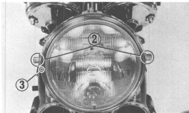
(2) Headlight mounting bolts (3) Beam adjusting screw
