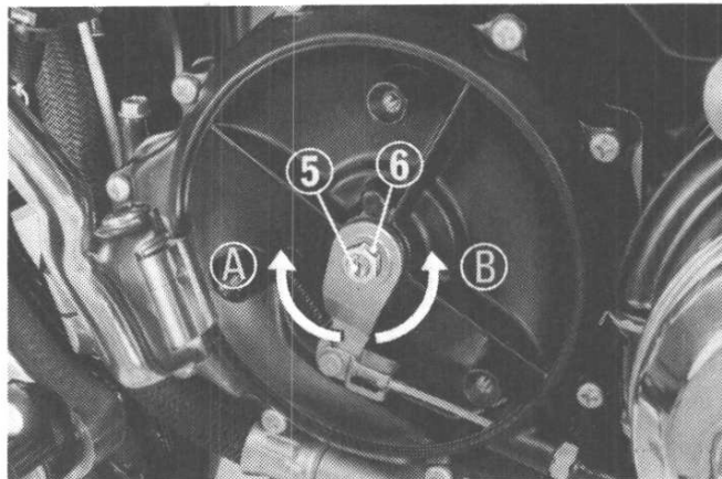
(5) Clutch adjusting screw (6) Adjusting screw lock nut
