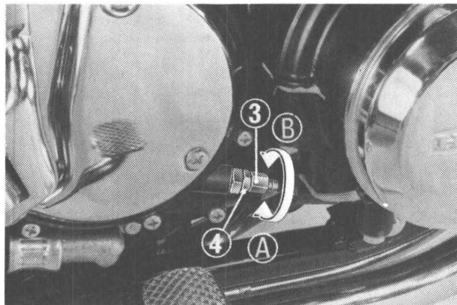
(3) Clutch cable adjusting bolt (4) Lock nut
