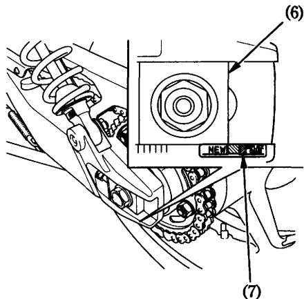
(6) Index mark
