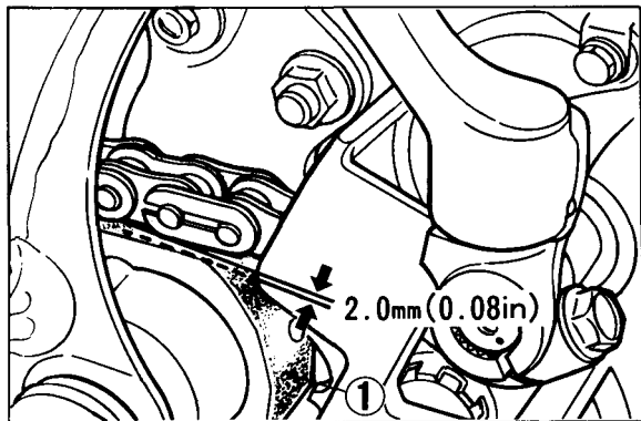
(1) Chain slider
